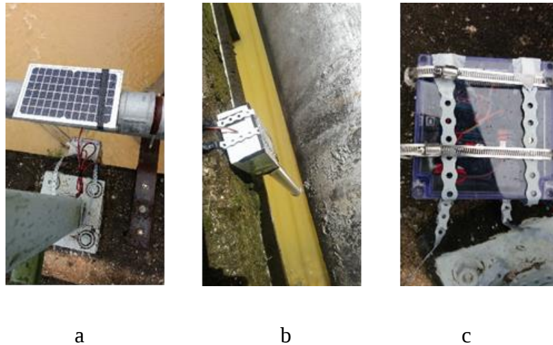
Figure 1.2: Mounting of sensor node done over river in Kemaman, Malaysia by Rodzi, Zakaria and Ismail (2017)
