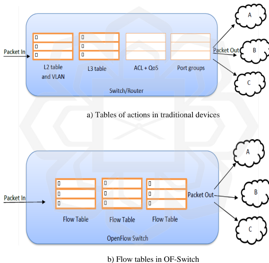
Figure 2.3: The difference in the internal structure of traditional and SDN devices
