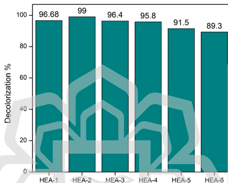
Figure 4.10 Degradation of Azo dye (methyl orange) with different composition of B in HEA milled powder as catalyst in the Fenton process
