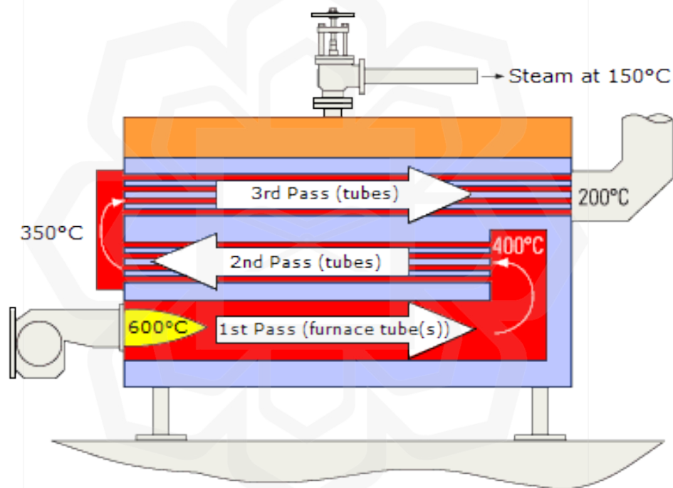
Figure 1.2 Shows the diagram of an industrial boiler process (Thermodyne, 2021).
